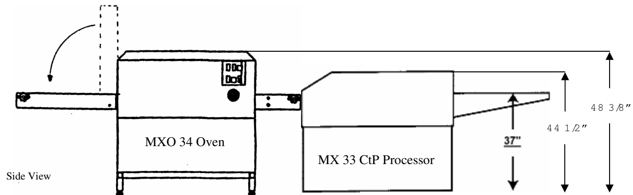
Installation Drawing MXO 34 Mini Oven On-Line with MX 33 CtP Plate Processor
